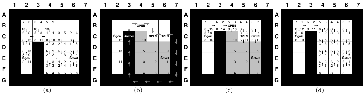
Figure 3: Example Search Problem with Changing Goal Cell
